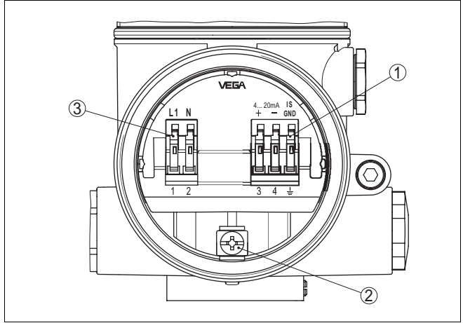
Fig. 9: Connection compartment, non-Ex instrument or Exd instrument
