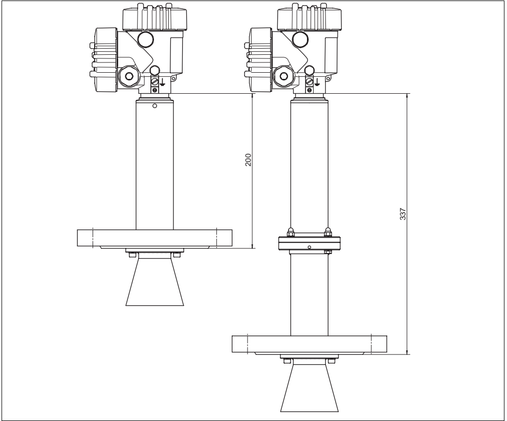
Fig. 17: VEGAPULS 66 for process temperatures up to 250°C or 400°C * dimension with integrated PLICSCOM
