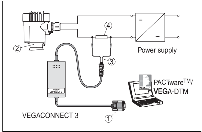
Fig. 14: PC connected to the signal cable
