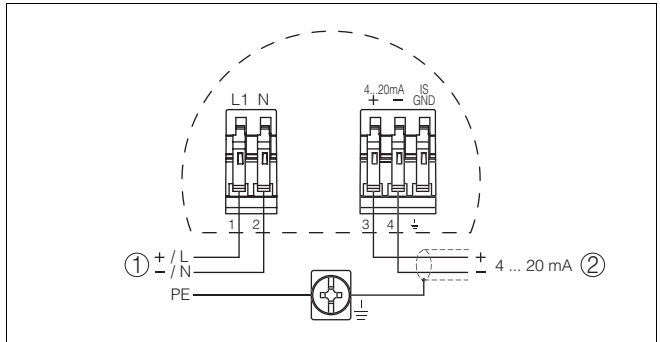
Fig. 10: Wiring plan, non-Ex instrument or Exd instrument
