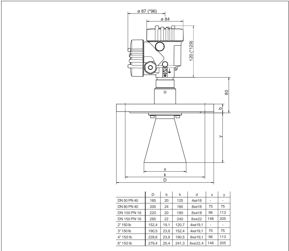
Fig. 16: VEGAPULS 66 in standard version
