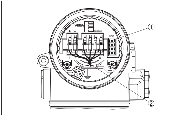
Fig. 8: Top view, electronics compartment, non-Ex instrument or Exd instrument
