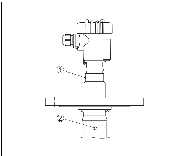
Fig. 4: Polarisation marking
