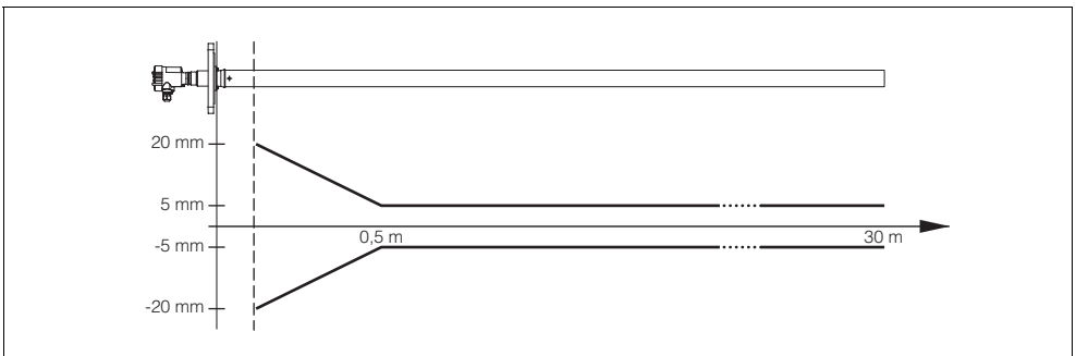
Fig. 15: Accuracy VEGAPULS 66
