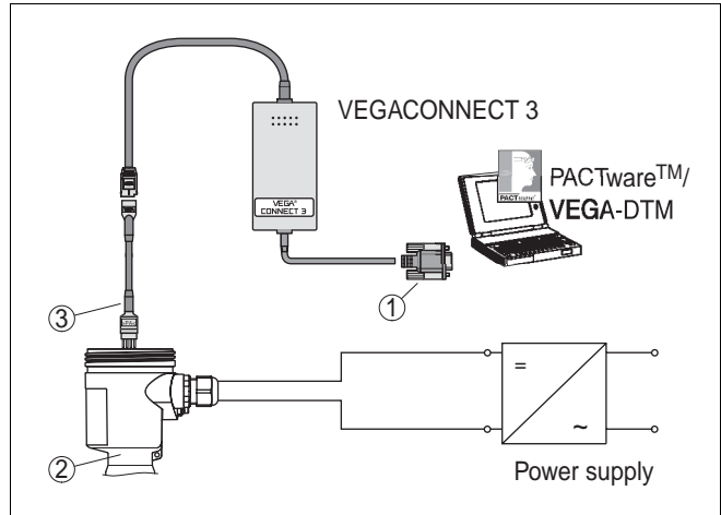
Fig. 13: PC connected directly to the sensor
